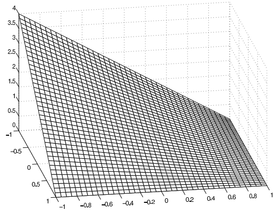
bilinear N_1(x)N_1(y)
