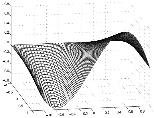
side shape fct. N_4(x)(1+y)
